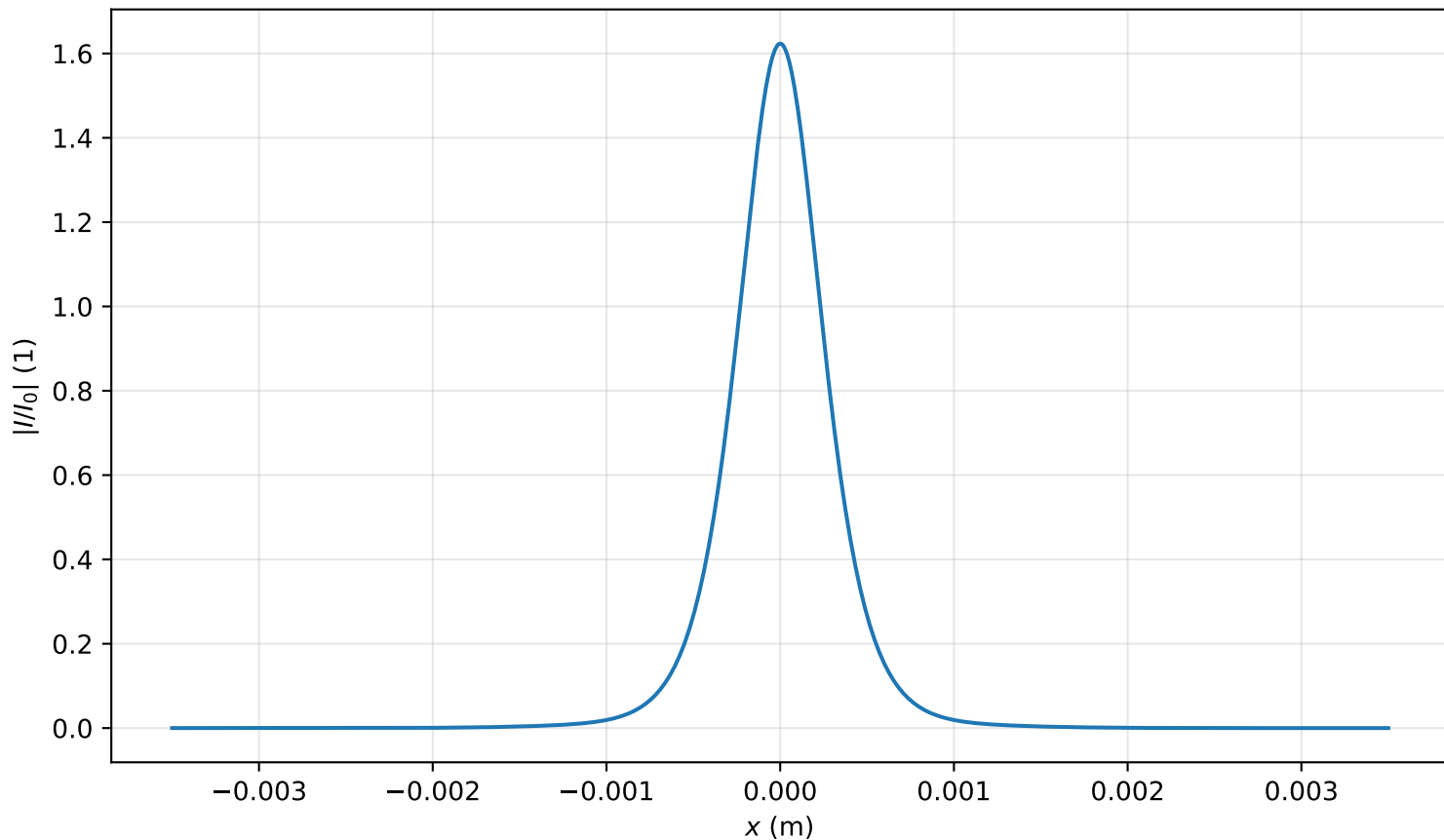
Intensity profile I(x, y = 0, z = 2.468m)/I_0 , P_{in}=0.9P_{cr} , artificial time
